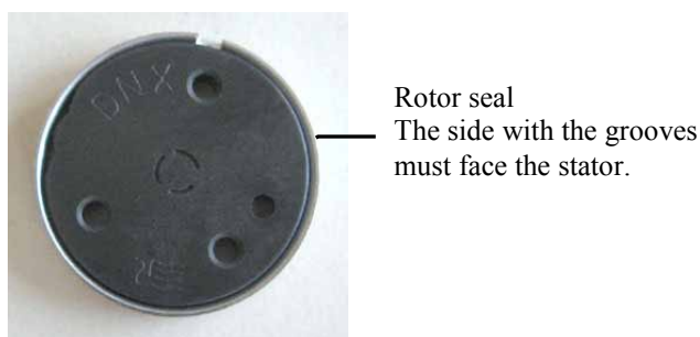
Fig. 53: Rotor seal
