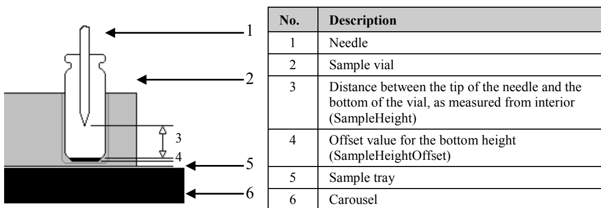
Fig. 39: Defining the needle height
